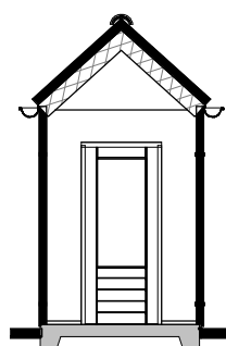
Doorsnede AS
